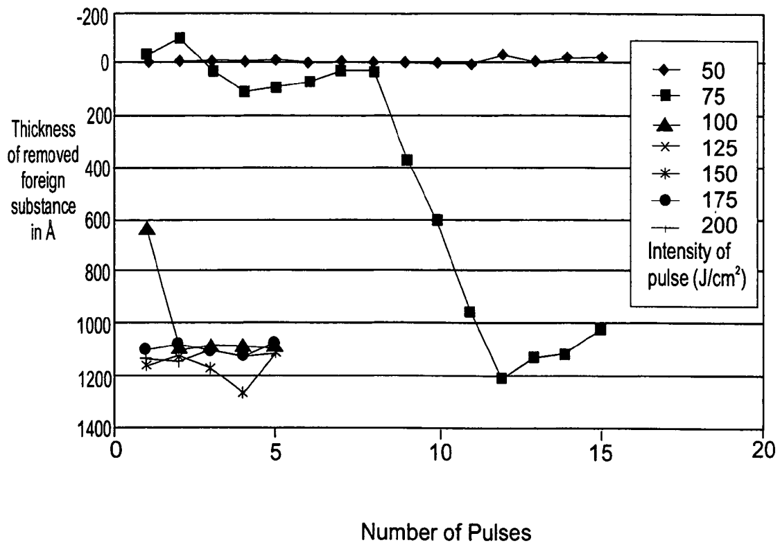
Laser Removal of Organic Emission Layer 150 on Auxiliary Layers 120/130
