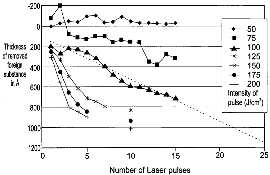
Laser Removal of Organic Emission Layer 150 absent Auxiliary Layers 120/130
